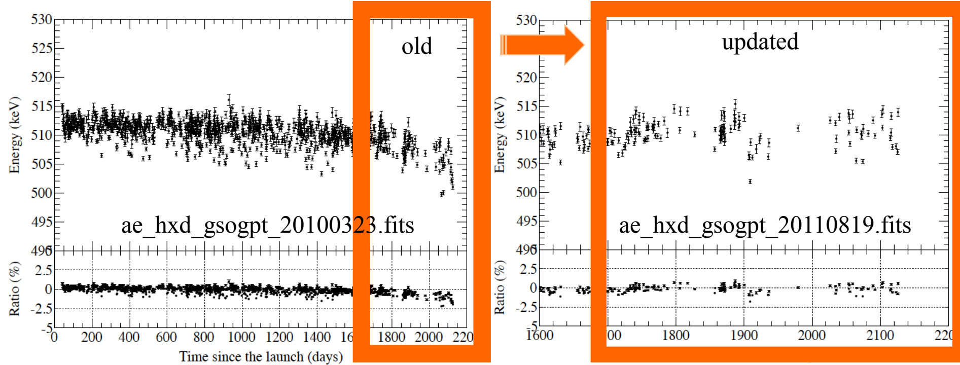
Gain History of all 16 units of GSO for a 511 keV line
