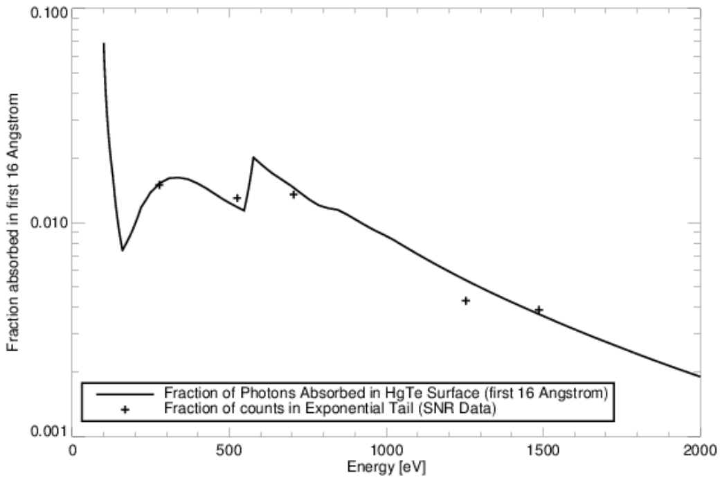
Figure 5 Absorption fraction as a function of photon energy in a surface layer on the HgTe absorbers (black solid line), plotted together with the fraction of events in the exponential tail (crosses).
