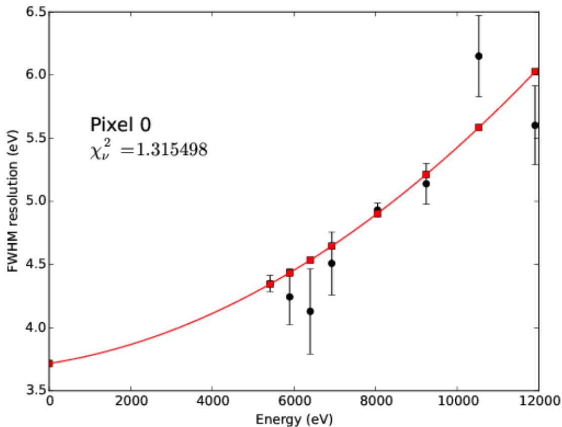
Figure 3. Measured and modeled FWHM resolution of HR events in Pixel 0. The measured points are from the calibration campaign in the FM Dewar in March 2015. The two data points with small error bars at 5415 eV and 8048 eV are from measurements with monochromators. The data point at 0 eV is from baseline events. The other data points are from deconvolution of fluorescence lines. The best-fit model is a quadratic function of energy.
