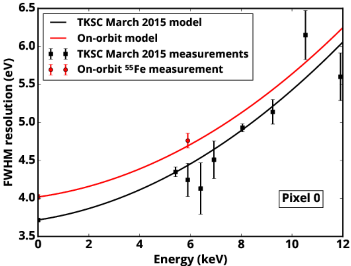
Figure 1. Resolution for hires events on pixel 0 (as in Figure 2), updated for on-orbit measurements of the baseline and 5.9 keV resolution.
