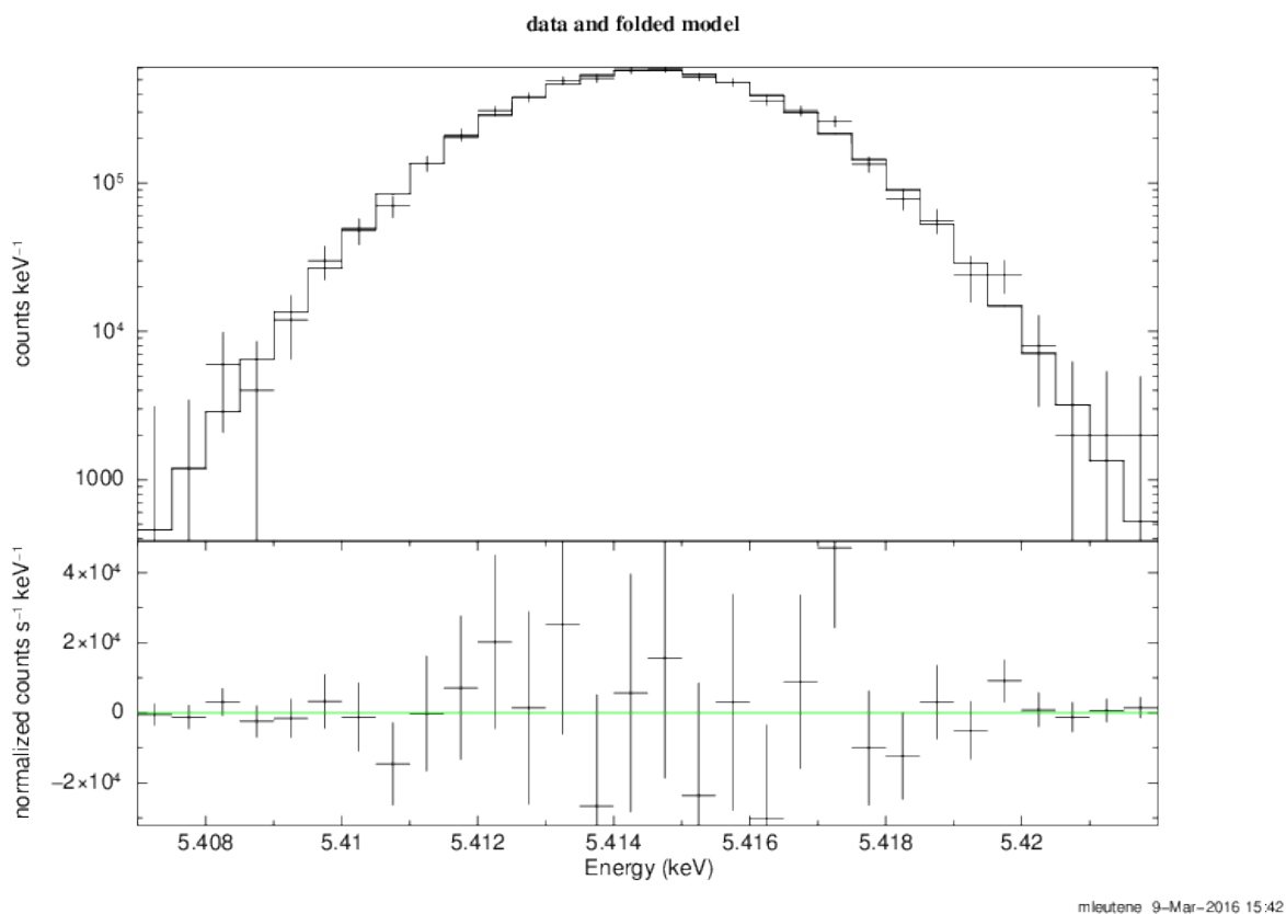
Figure 2. Gaussian fit to the observed spectrum of pixel 3 HR events from an experiment with a monochromator at 5415 eV. The FWHM of the monochromator is 0.24 eV.
