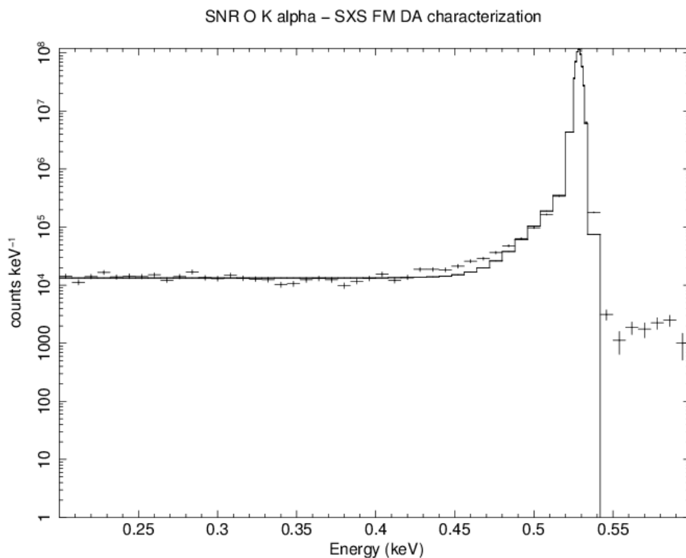
Figure 4 We show an example of a fit to data acquired with monochromatized O K shell fluorescence line emission in Figure 1. The core of the LSF is modeled with a Gaussian, and the tail is modeled with a flat (in energy) continuum to represent the electron loss continuum, and an exponential to represent energy lost to long-lived surface excitations. No significant escape peaks are present for incident photons with energies below the Hg M ionization threshold at 2295 eV. The tail on the high energy side of the line is an artifact of the monochromator.
